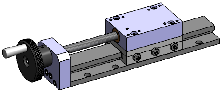
MODEL NAME: Gen2 SLIDE with LEAD SCREW CONFIG: SW02-SL03-BL08-LS
