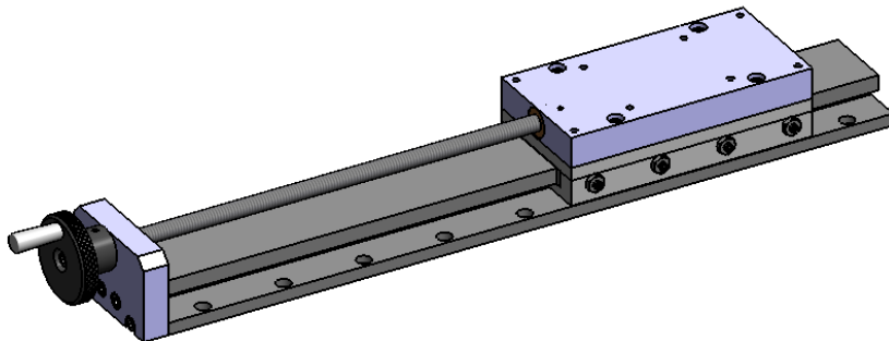
MODEL NAME: Gen2 SLIDE with LEAD SCREW CONFIG: SW03-SL06-BL18-LS
